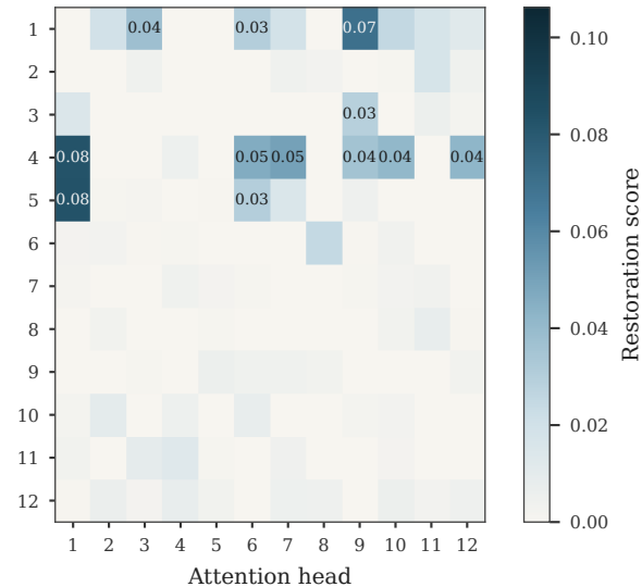
Recovery (BNC)
